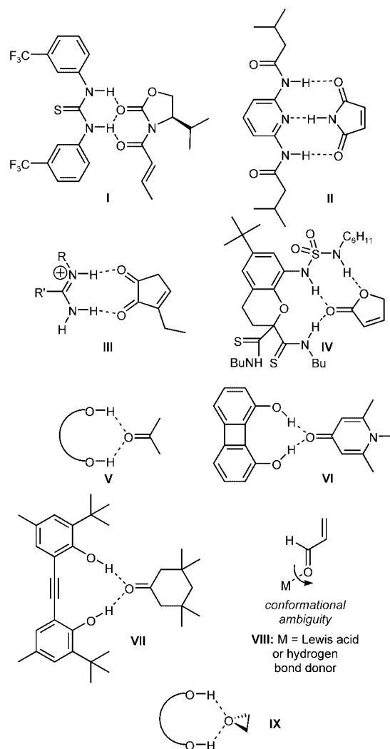
Figure 1. Hydrogen bonded complexes.
