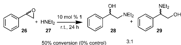
Scheme 8. Epoxide ring-opening catalysed by PHANOL 1 .
