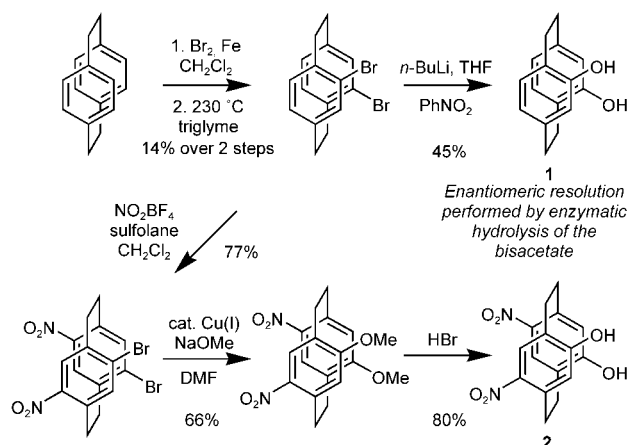
Scheme 1. Synthesis of PHANOLs 1 and 2 .
