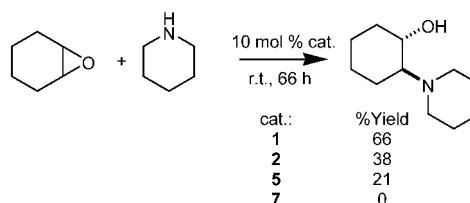
Scheme 9. Epoxide ring-opening catalysed by PHANOLs.
