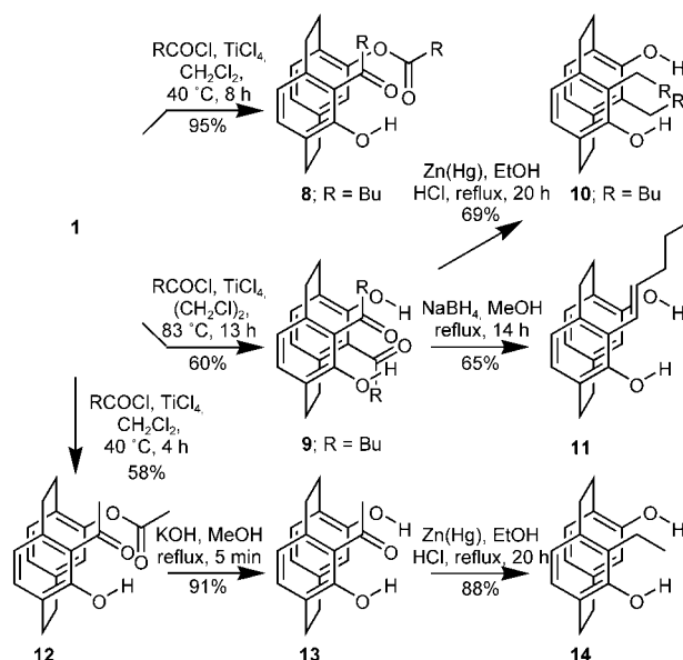
Scheme 3. Synthesis of PHANOLs 10 , 11 and 14 .
