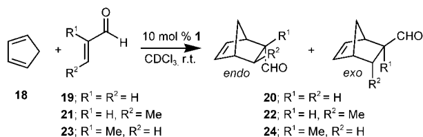
Scheme 6. Diels–Alder reactions catalysed by PHANOL 1 .
