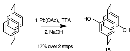
Scheme 4. Synthesis of PHANOL 15 .
