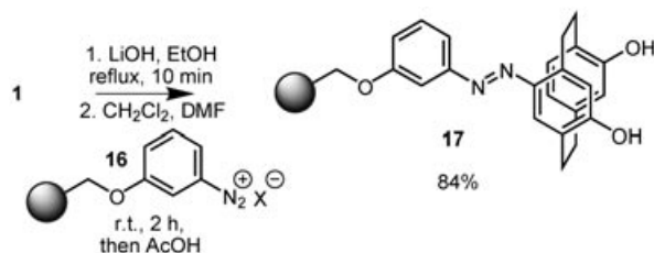
Scheme 5. Synthesis of polymer-supported PHANOL 17 .
