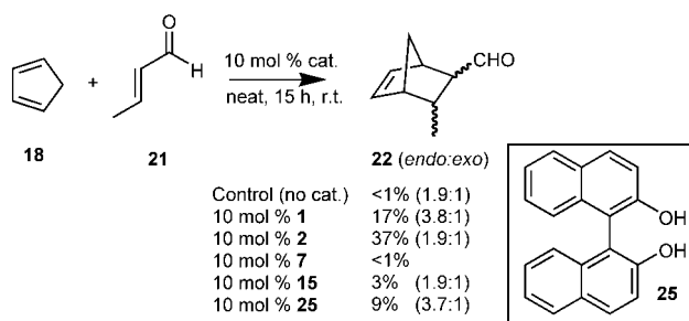
Scheme 7. Diels–Alder reaction catalysed by PHANOLs.
