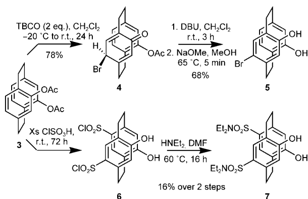
Scheme 2. Synthesis of PHANOLs 5 and 7 .
